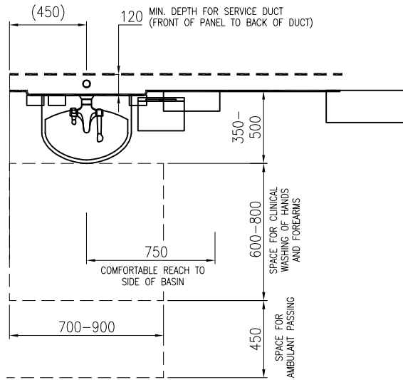
PLAN: CONCEALED SERVICE DUCT
