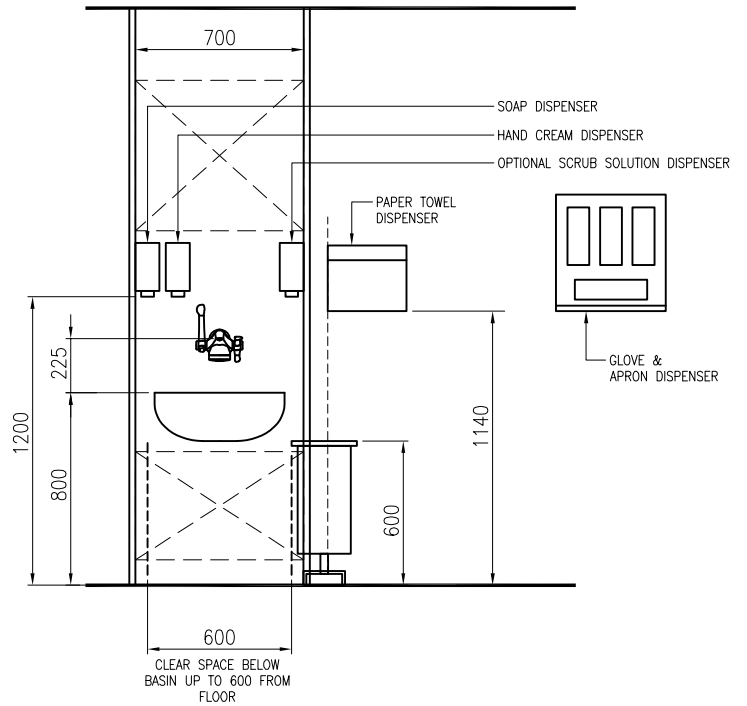
ELEVATION: PROJECTING SERVICE DUCT
